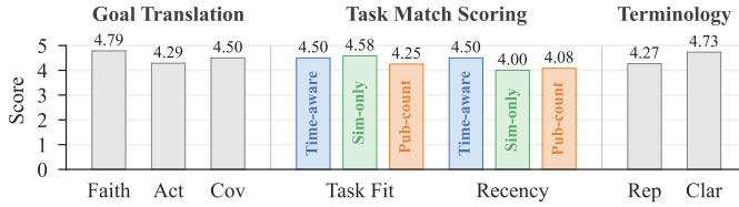
Fig. 7. Mean expert-user ratings for the evaluated goal translation, task match scoring, and terminology comparison outputs.
